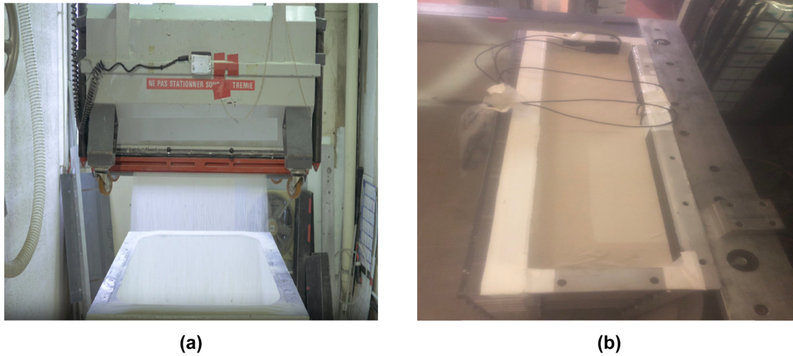
Figure 1. Sand preparation process: (a) sand raining technique and (b) prepared strongbox.
