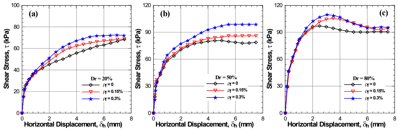
Figure 8: Effect of polypropylene fibre content on sand shear strength ( \sigma_n = 100 kPa): (a) Dr = 20\% , (b) Dr = 50\% and (c) Dr = 80\% . Dr , relative density.
