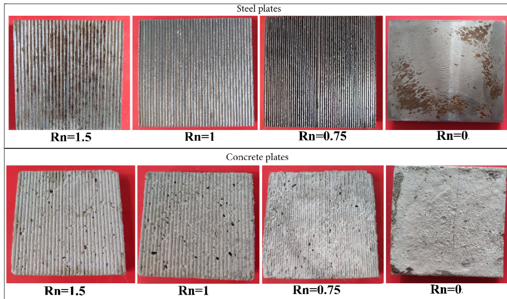
Figure 2: Steel and concrete plates with various Rn values.
