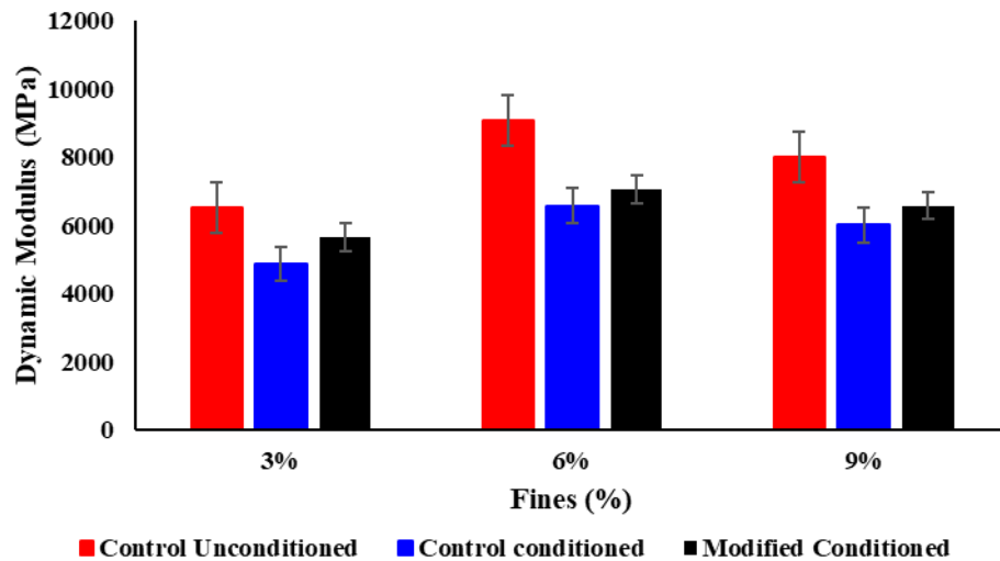
Figure 4: Measured dynamic modulus of asphalt concrete mixtures with 3%, 6%, and 9% fines with and without freeze–thaw conditioning.
